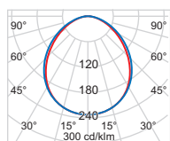
T5 1 x 54 W UGR 19,1 / 19,6 Critical radiation angle/1000 cd/m 2 90° Light output ratio 57%
