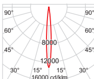
HIT-CE 35 W Half-value angle 2 x 6° Light output ratio 83%
