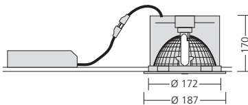
HIT-CE 35 W Half-value angle 2 x 6° Light output ratio 83%
