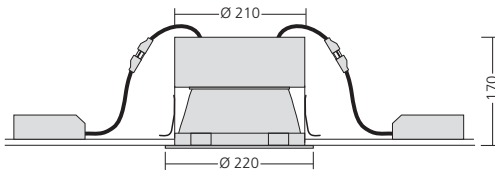
HIT-CE 2 x 35 W Half-value angle 2 x 41° Light output ratio 57%
