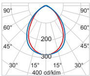
HIT-CE 2 x 35 W Half-value angle 2 x 41° Light output ratio 57%
